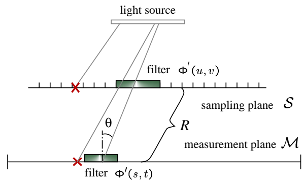
Figure 2: Cross section through the conceptual acquisition setup.
