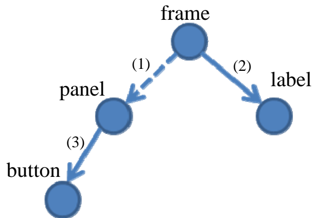
Figure 6: High level illustration of a dynamic model (object graph) including design (solid) and dynamic (dotted line) information. Numeric labels refer to “add” relationships between widgets in Figure 7. Design model will appear to the user as truncated version of dynamic model.
