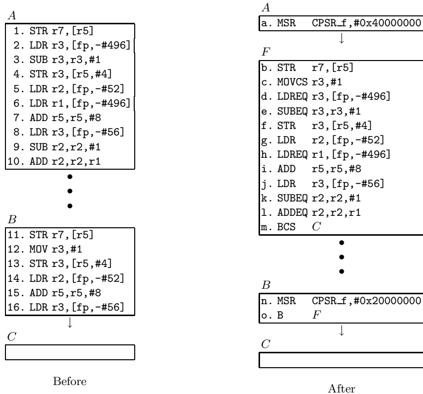
Fig. 4. Abstraction of two blocks from an ARM executable. The predicated branch instruction (instruction m) permits block A to fall-through (↓) to F and continue after F without branching to C.
