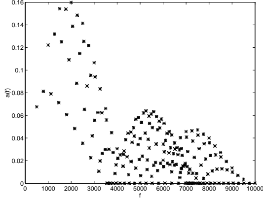
Figure 5: Square membrane struck at (0.1, 0.1) .
