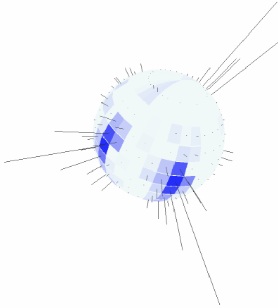
Figure 3: Pressure distribution measurements on the Tango during a three finger grasp. Higher pressures are indicated by darker taxels and longer arrows.
