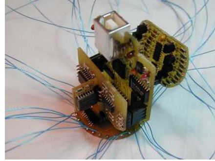
Figure 2: Sensing and communication electronics.
