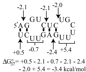
Fig. 1. Secondary structure of an RNA strand of length 20. An RNA molecule, or strand, is a sequence of Adenine (A), Cytosine (C), Guanine (G), or Uracil (U) bases, with two chemically distinct ends, known as the 5' and 3' ends. The secondary structure is the set of base pairs (indicated by black boxes) that form when the molecule folds, under fixed environmental conditions. Throughout, we consider only pseudoknot-free secondary structures. The base pairs give rise to loops . The depicted structure includes a hairpin loop (right end of diagram), as well as three base pair stacks and a 2 \times 2 internal loop. In the Turner99 model, the total free energy change of a structure, relative to its unfolded state, is the sum of the free energy changes of its loops. The lower the free energy change, the more stable the structure. Generally, stacked base pairs tend to stabilize the RNA structure, whereas loops with unpaired bases are destabilizing. In the depicted structure, contributions to the total free energy change at 37°C, denoted by \Delta G_{37}^0 (measured in kcal/mol), include a +5.4 penalty for closing the hairpin loop, which is largely an entropic cost, a -2.4 favourable term for the rightmost (UA/CG) stacked pair, and a +0.5 penalty for an AU pair at the end of a helix (as well as other terms).
