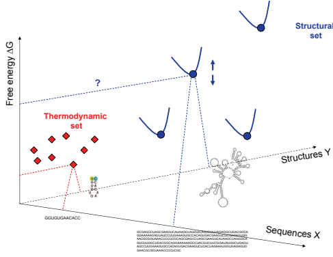
Fig. 2. Schematic representation of the structural and thermodynamic data sets we use in our constraint generation algorithm. The X and Y axes represent RNA sequences and secondary structures, respectively. The diamonds on the left represent (x, y_x, e_x) triples that form the thermodynamic set, while the dots on the right represent (x, y_x) pairs forming the structural set. The curves depict the fact that the known y_x structures from the structural set have lower free energy change than any other structure into which x can fold, although we do not know where these points are situated on the vertical free energy axis.
