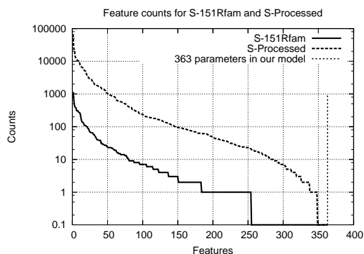
Fig. 6. The feature counts for various structural sets (features are ordered according to decreasing counts). Out of the 363 total parameters, only 254 appear at least once in S-151Rfam, and 348 appear at least once in S-Processed. The thermodynamic set T-Full contains 203 features out of all 363 features in the model.
