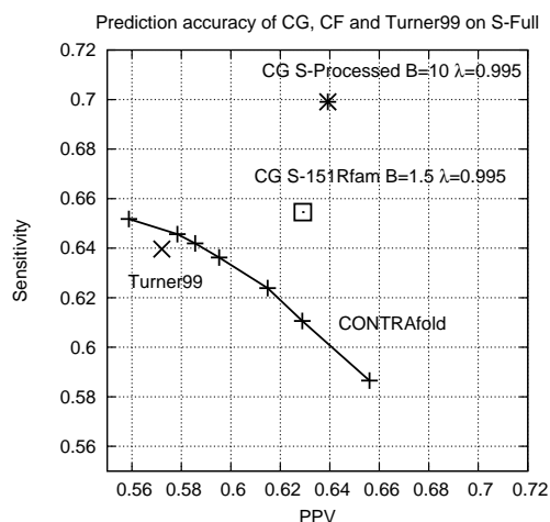
Fig. 8. RNA secondary structure prediction accuracy obtained when using the Turner99 parameters, CONTRAfold parameters ( \gamma \in \{2, 3, 4, 6, 8, 10, 20\} ) and CG parameters (trained on S-151Rfam and S-Processed). Tested on a wide range of biological RNA structures in set S-Full, the parameters obtained using CG give significantly better accuracy than those found by CONTRAfold and the Turner99 parameters.
