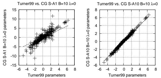
Fig. 5. Correlation between “true” Turner99 parameters and estimated parameters on the artificial training set when the feature coverage k (minimum number of times each feature occurs in the set), is 1 (left) and 10 (right). When k = 10 , the estimated parameters are very close to the “true” ones.
