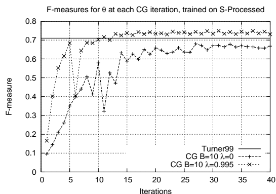
Fig. 7. F-measure when trained on S-Processed vs iteration number for the CG algorithm. Usually the accuracy at the first iterations is much lower than the accuracy of the initial parameter set used (i.e., the Turner99 set), because the number of inequality constraints is small. The algorithm usually converges in about 20 iterations.
