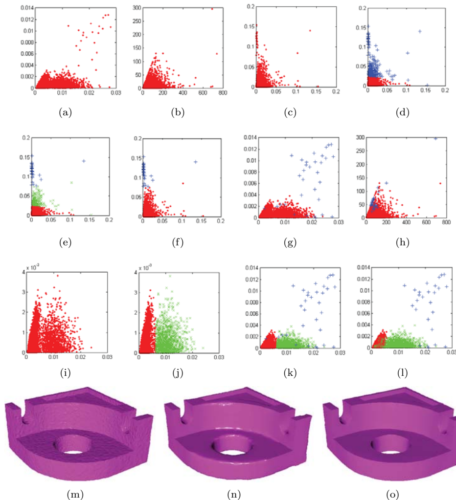
FIG. 9. (a) Height intensity data matrix H computed for the noisy bearing model in (m); (b) principal curvature data matrix C ; (c) scaled Gaussian curvature data matrix G ; (d) two clusters in G classified by K -means; (e) reclassifying the corner cluster (blue) in (d) by K -means; (f) replacing the corner cluster in (d) with new corner cluster generated in (e) and combining new noncorner cluster (green) with old noncorner cluster in (d); (g) locating corner vertices identified by Gaussian curvature in (a); (h) locating corner vertices in (b); (i) temporarily removing the corner cluster from (g); (j) two clusters by K -means for the data that has remained in (i): red \rightarrow nonfeature and green \rightarrow edge; (k) adding the corner cluster back into (j); (l) classification refinement; (m) noisy bearing model; (n) smoothed model based on the vertex partition in (k); (o) smoothed model based on the refined vertex partition (l).
