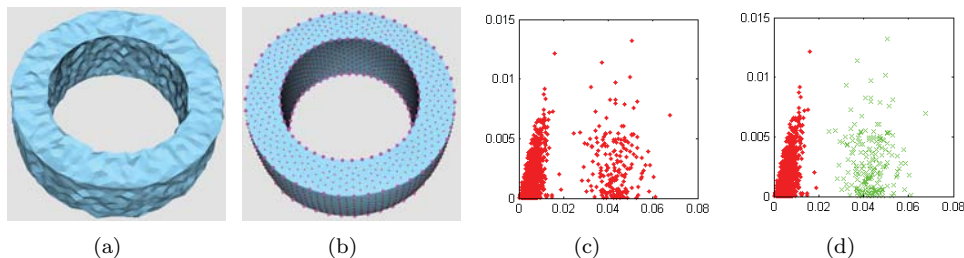
FIG. 3. (a) Corrupted ring model ; (b) smoothed model based on partition in (d): nonfeature vertices are marked by smaller pink dots and feature (edge) vertices are marked by larger pink dots ; (c) data set H computed for the noisy ring model in (a) ; (d) two clusters by K-means: red \rightarrow nonfeature and green \rightarrow feature .
