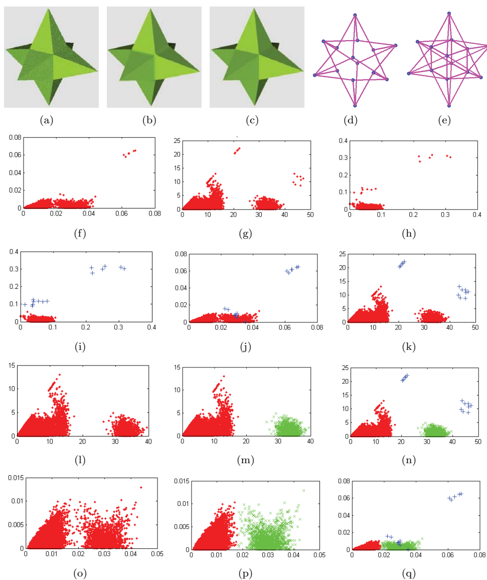
FIG. 4. (a) Corrupted star model; (b) smoothed model based on partition in (n); (c) smoothed model based on partition in (q); (d) 3D plot of feature vertices classified by principal curvatures (blue and green clusters in (n)); (e) 3D plot of feature vertices classified by height intensities (blue and green clusters in (q)); (f) data set H computed for the noisy Star model in (a); (g) data set C ; (h) data set G ; (i) two clusters by K -means on data set G for corner identification: blue \rightarrow corner; (j) marked corner vertices classified by Gaussian curvature in data set H ; (k) marked corner vertices in data set C ; (l) temporarily removing the corner cluster from data set C ; (m) two clusters by K -means on data that have remained in (l): red \rightarrow nonfeature and green \rightarrow edge; (n) adding the corner cluster back into (m); (o)–(q) same process as (l)–(n) but performed on data set H instead.
