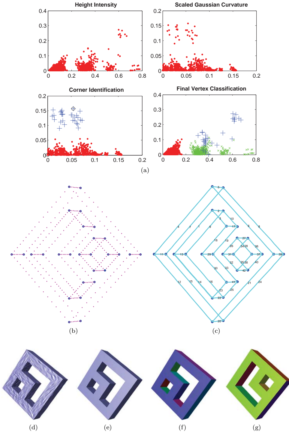
FIG. 11. (a) Vertex classification for the noisy torus model in (d); (b) 3D plot of edge and corner vertices based on clusters in (a); (c) crease detection; (d) noisy torus model; (e) smoothed model based on the vertex partition in (a); (f) mesh segmentation (16 patches) when all detected creases in (c) are input to construct cutting paths; (g) another view of (f).
