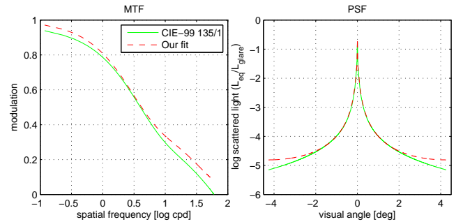
Figure 3: Comparison of our fitted intra-ocular light scatter model with the model from the CIE-99 135/1 report [Vos and van den Berg 1999]. Left panel shows the modulation transfer function of the eye and the right panel its corresponding point spread function. The MTF for the CIE-99 135/1 glare spread function has been computed by creating a densely sampled digital filter and applying the inverse Fourier transform.
