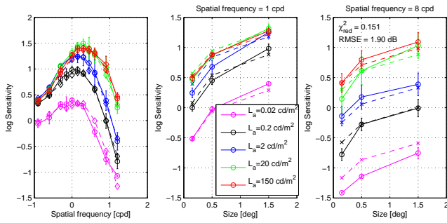
Figure 8: Visual model predictions for the CSF for wide luminance range data set. The two plots on the right show sensitivity variation due to stimuli size.
