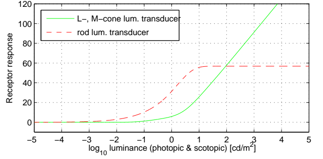
Figure 5: The luminance transducer functions for cones ( t_L = t_M ) and rods ( t_R ).
