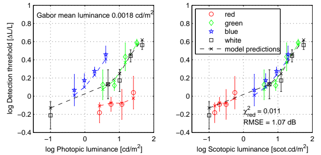
Figure 10: Visual model predictions for the color glare at scotopic levels data set. The leftmost point represent the threshold without glare source.
