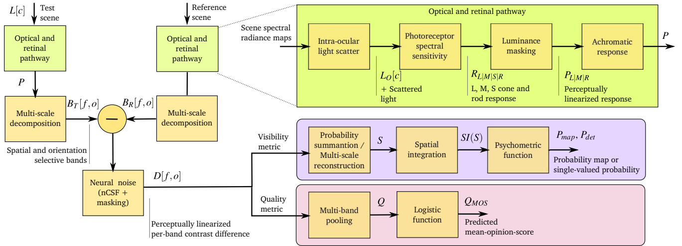
Figure 2: The block-diagram of the two visual metrics for visibility (discrimination) and quality (mean-opinion-score) predictions and the underlying visual model. The diagram also summarizes the symbols used throughout the paper.
