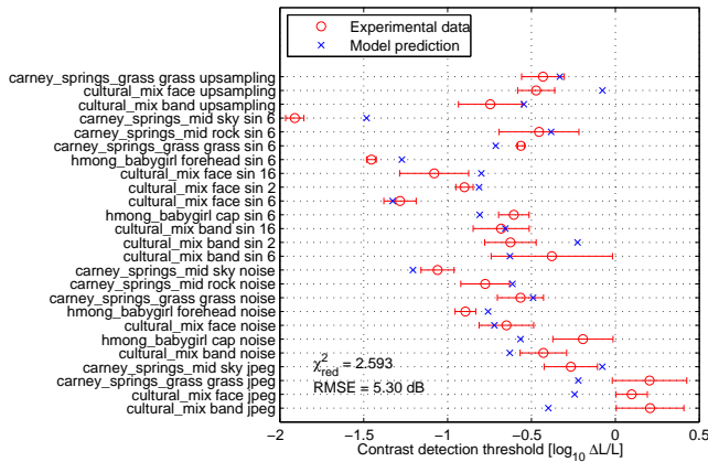
Figure 12: Visual model predictions for the complex images data set.
