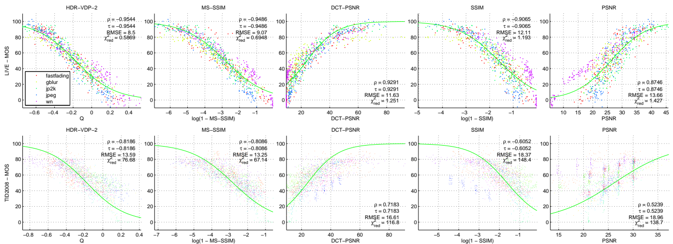
Figure 13: Predictions of quality metrics for the LIVE (top) and TID2008 (bottom) databases. The prediction accuracy is reported as Spearman's \rho , Kendall's \tau , root-mean-square-error (RMSE), and the reduced \chi^2 statistics. The solid line is the best fit of the logistic function. Only the LIVE database was used for fitting. See supplementary for enlarged and more detailed plots.
