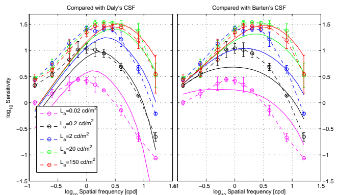
Figure 6: The CSF measurement results compared to two popular CSF models by Daly [1993] and Barten [1999]. The Dashed lines represent our measurements and the solid lines the two compared models. The model parameters, including stimuli size, were set to match our measurements. The predictions of both models differ from the measurements probably because of different experiment conditions.
