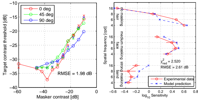
Figure 11: Visual model predictions for the Foley's masking data [Foley 1994] on the left and CSF flattening data set on the right. The degree values in the legend correspond to the orientation of the masking pattern with respect to the test pattern (0 deg. - vertical).
