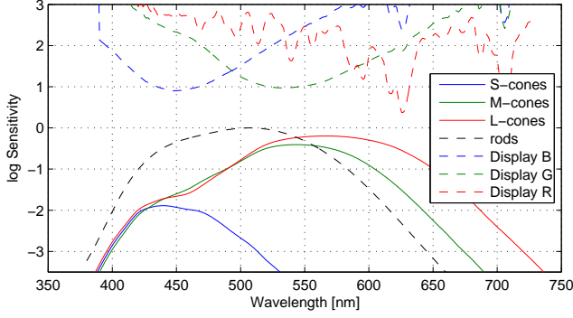
Figure 4: Spectral sensitivities of the photoreceptors from [Stockman and Sharpe 2000] and [CIE 1951] (bottom). The curves in the upper part of the plot show the measured emission spectra for a CRT display (inverted and arbitrarily scaled to distinguish from the bottom plots).
