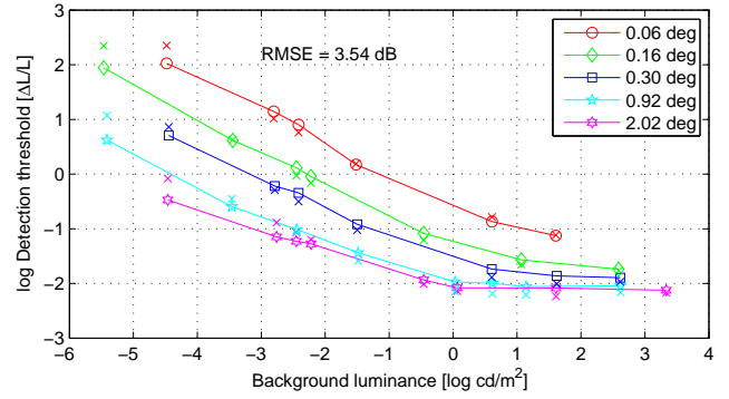
Figure 9: Visual model predictions for the threshold versus intensity curve data set. These are the detection thresholds for circular patterns of varying size on a uniform background field [Blackwell 1946].
