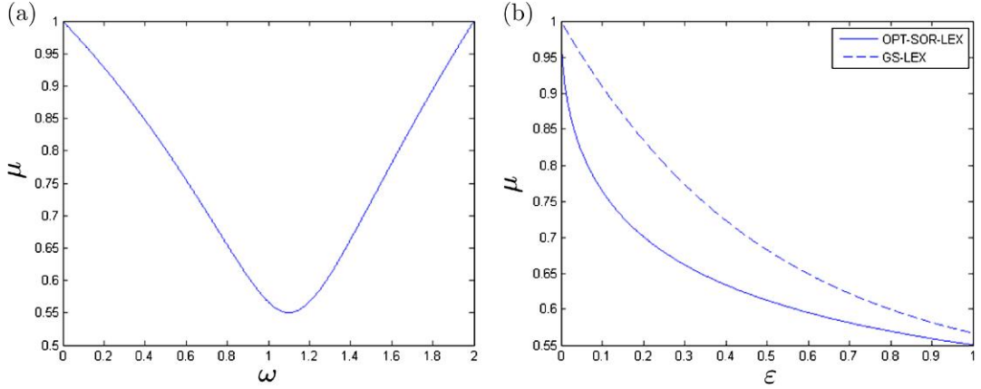
FIG. 4. Left: Smoothing factor of SOR-LEX with relaxation parameter \omega , as a function of \omega , for the standard seven-point centred-difference discretization of the three-dimensional Poisson problem. Right: Smoothing factors of GS-LEX and optimal SOR-LEX applied to the anisotropic diffusion problem -\epsilon u_{xx} - u_{yy} - u_{zz} = f , as a function of \epsilon , assuming seven-point centred-difference discretization.
