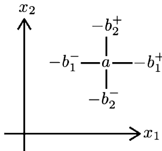
FIG. 1. The computational molecule associated with the operator \mathcal{L}^h ( d = 2 ).
