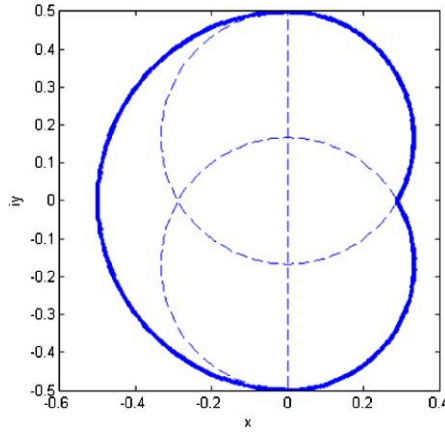
FIG. 3. The heart-shaped set D is the union of two disks and a half disk.
