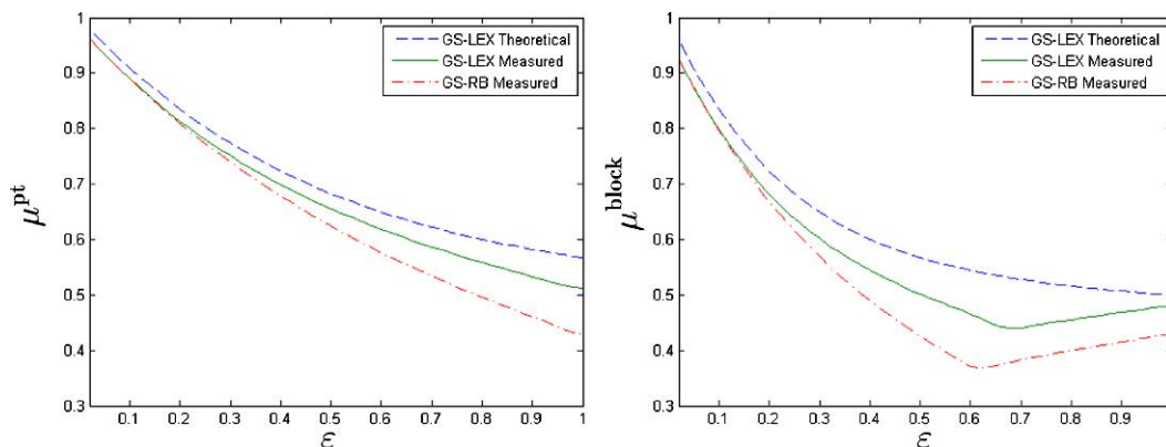
FIG. 5. Theoretical smoothing factors of GS-LEX versus experimental asymptotic convergence rates of two-level multigrid with GS-LEX and GS-RB smoothers, applied to the steady-state diffusion equation -u_{xx} - u_{yy} - \epsilon u_{zz} = f . Pointwise relaxation appears on the left, while x -oriented line relaxation is depicted on the right. The discretization is on a 23 \times 23 \times 23 grid with centred differences.
