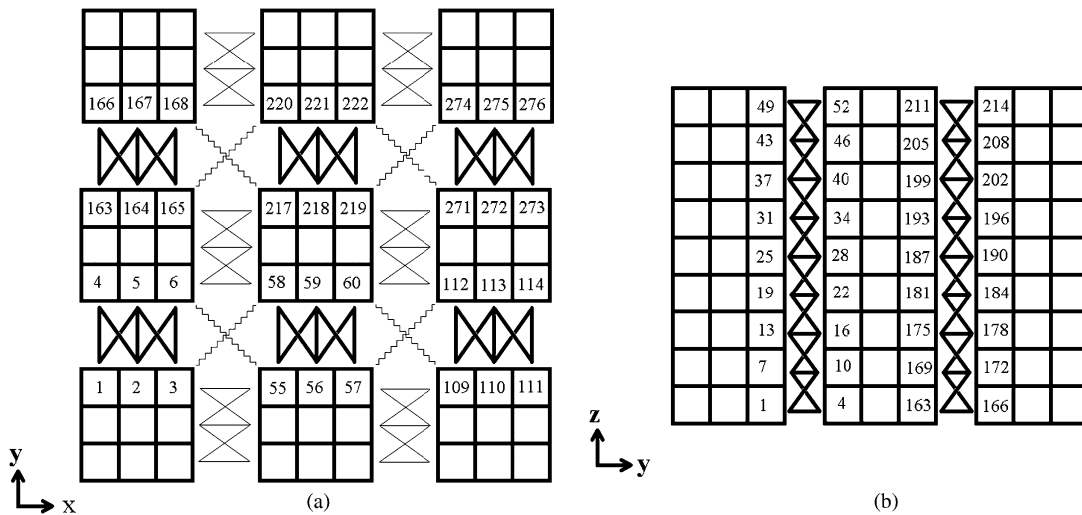
Figure 7. (a) A z =constant slice of the graph of N_{kP} for a 9 \times 9 \times 9 grid with k=3 and (b) A x =constant slice.
