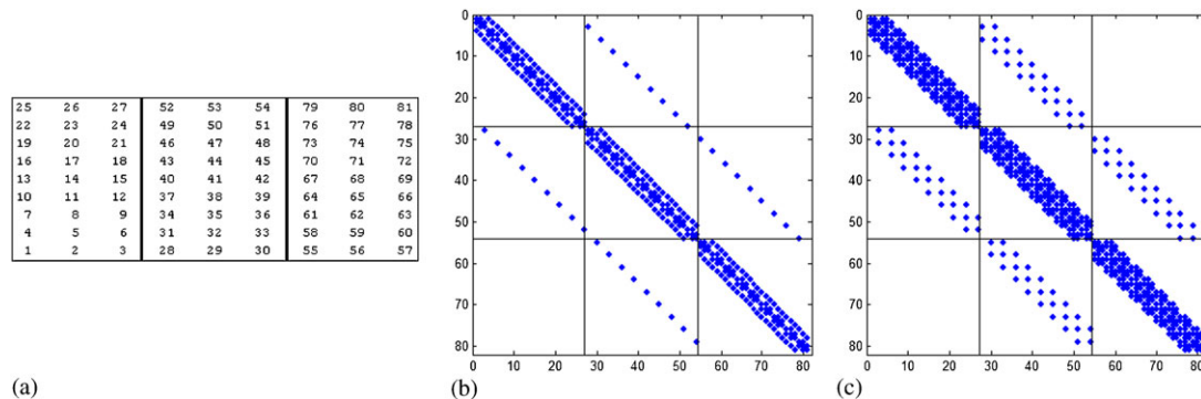
Figure 3. (a) 3-line ordering applied to a 9 \times 9 grid. The grid blocks are separated by lines; (b) The induced block structure of the 5-point operator matrix; and (c) The induced block structure of the 9-point operator matrix.
