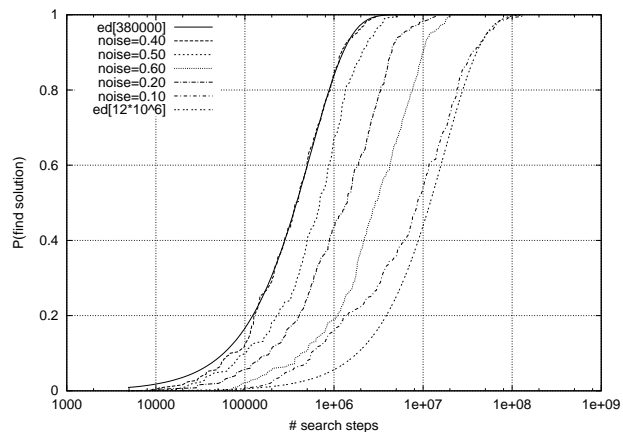
Figure 1: Left : Noise response for Novelty + on easy, medium, and hard instances from test-set flat100-239-100. Right : RTDs for for WalkSAT/SKC on SAT-encoded block world planning instance bw_large.b for approx. optimal, lower and higher noise settings.
