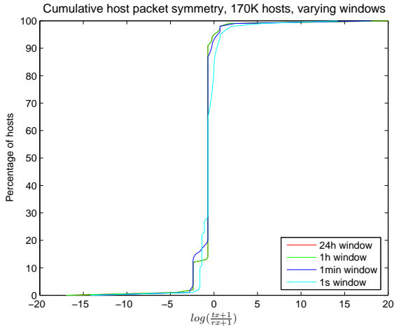
Figure 4: Host Symmetry
