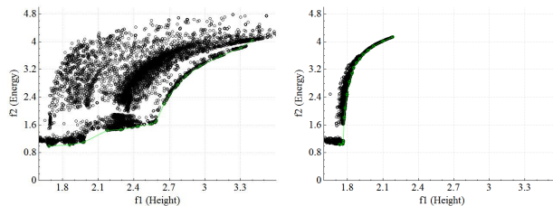
(a) Re-sampling with a success rate of 13/16
