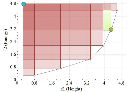
Figure 5: Hypervolume sorting. The blue point is a reference point chosen to be worse off than all possible samples in all objectives. The red regions show the area (Lebesgue measure in 2D) of rectangles (hyper-cuboids in 2D) specified by a sample on the Pareto-optimal front and the reference point. The green region denotes the area contribution (hypervolume contribution in 2D) of the green non-dominated sample on the Pareto-optimal front.
