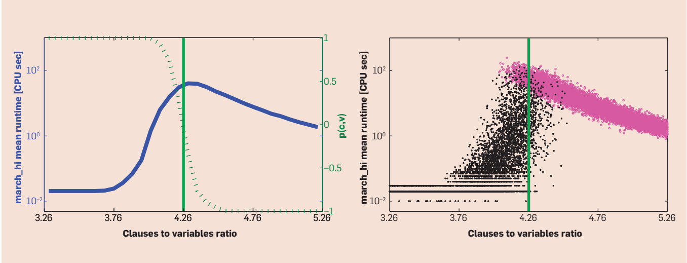
Figure 1. Runtime of march_hi on uniform-random 3-SAT instances with v = 400 and variable c/v ratio. Left: mean runtime, along with p(c, v) ; right: per-instance runtimes, colored by satisfiability status. Runtimes were measured with an accuracy of 0.01s, leading to the discretization effects visible near the bottom of the figure. Every point represents one SAT instance.
