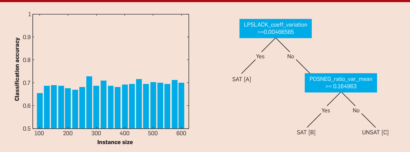
Figure 3. Left: Classification accuracies for our simple decision tree on uniform-random 3-SAT instances at the phase transition with varying numbers of variables. The tree was trained only on 100-variable data. Right: The decision tree. Predictive accuracies for instances falling into the three regions were between 60% and 70% (region A); about 50% (region B); and between 70% and 80% (region C).
