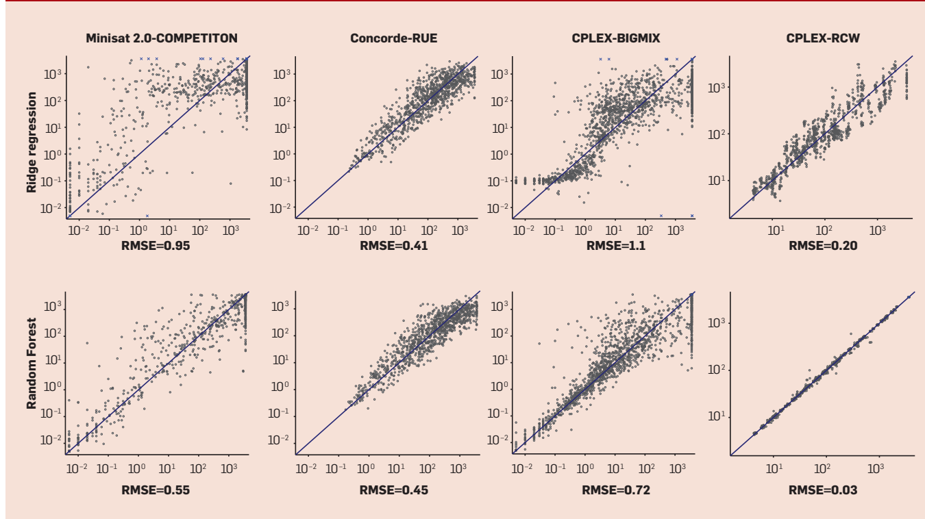
Figure 4. Visual comparison of models for runtime predictions on unseen instances. In each plot, the x-axis denotes true runtime and the y-axis runtime as predicted by the respective model. Predictions above 3,000 or below 0.001 are denoted by a blue x.
