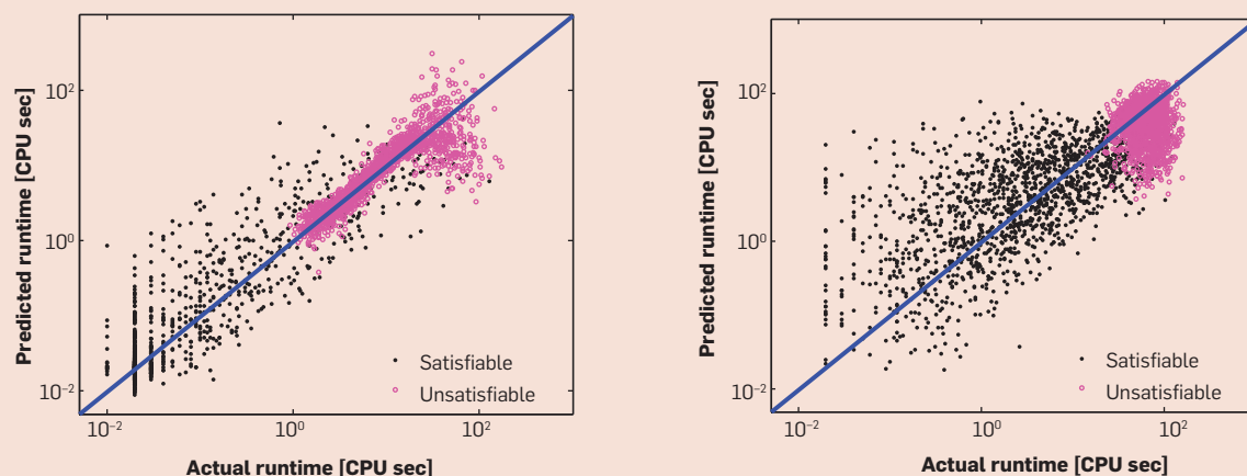
Figure 2. Actual vs. predicted runtimes for march_hi on uniform-random 3-SAT. Each dot represents a test instance not used to train the model; perfect predictions would fall along the diagonal. Left: c/v \in [3.26, 5.26] ; Right: c/v = 4.26 .
